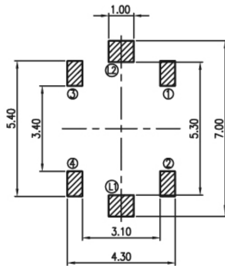
PCB layout
